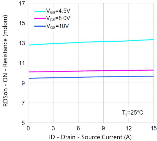
Figure 3. Rdson-Drain Current
