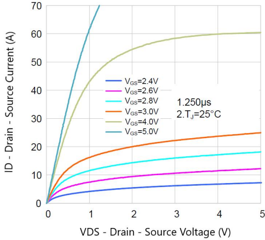
Figure 1. Typ. Output
