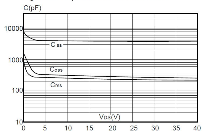
Figure 6: Capacitance Characteristics
