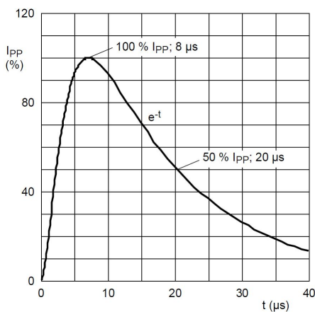
8/20 µs pulse waveform according to IEC 61000-4-5
