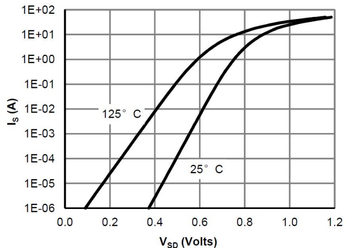
Figure 6: Body-Diode Characteristics
