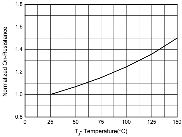
Figure 7. R ds(on) -Junction Temperature(°C)
