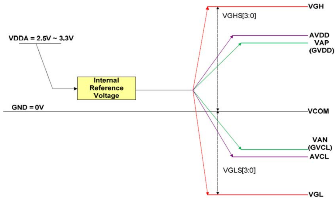
Fig.2 Voltage Generation
