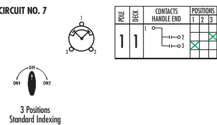
CIRCUIT NO. 7
