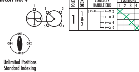
CIRCUIT NO. 4
