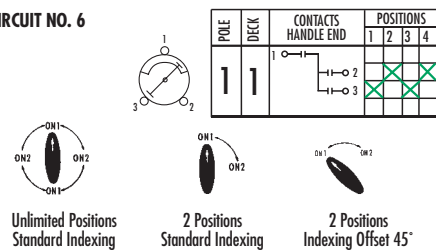
CIRCUIT NO. 6
