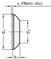
Plastic disc
