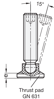
Mounting example
