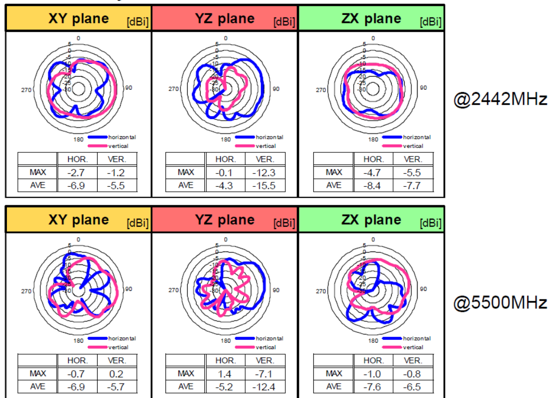
Figure 12 – Directivity for 1LV M.2 Module Mounted on iMX OEM Carrier Board
