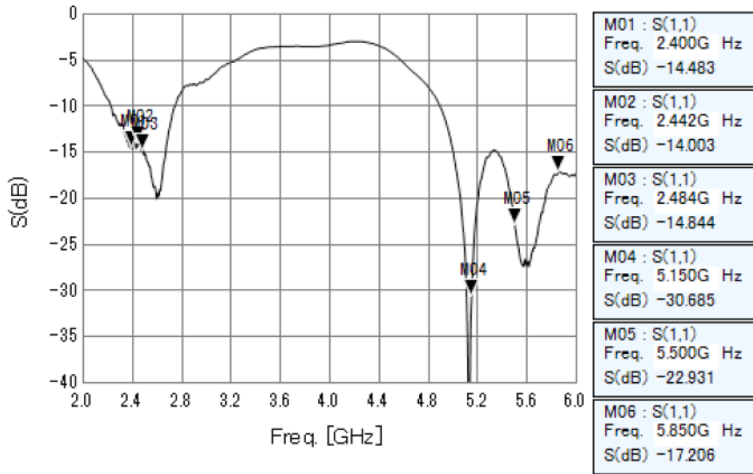
Figure 10 – Return Loss for 1LV M.2 Module Mounted on iMX OEM Carrier Board
