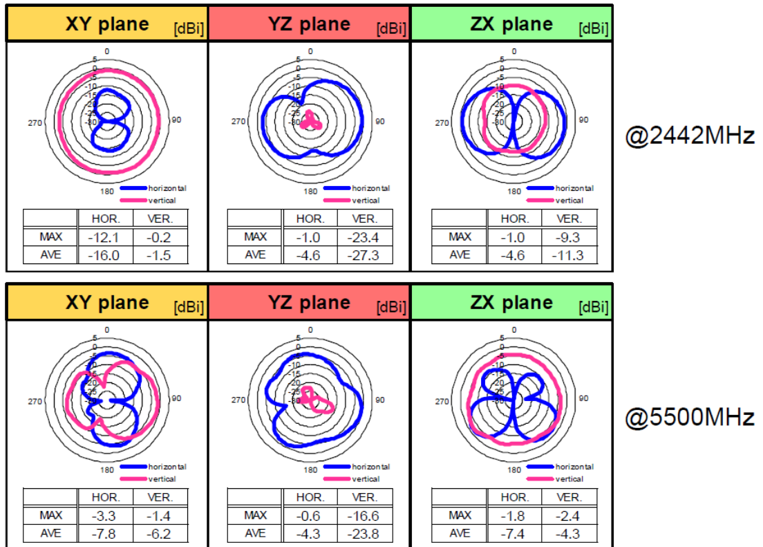
Figure 15 – Directivity for 1LV M.2 Module Standalone
