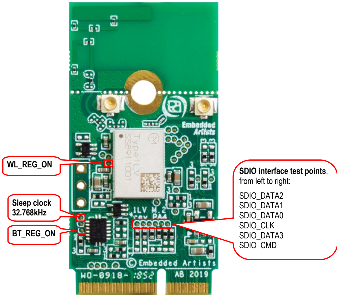
Figure 4 – 1LV M.2 Module Test Points
