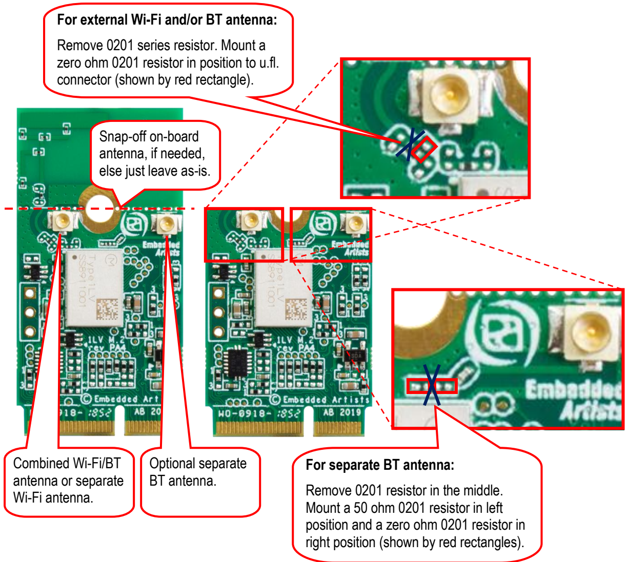
Figure 6 – Rework to Connect U.FL. Connectors
