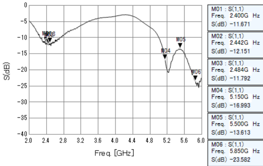
Figure 13 – Return Loss for 1LV M.2 Module Standalone
