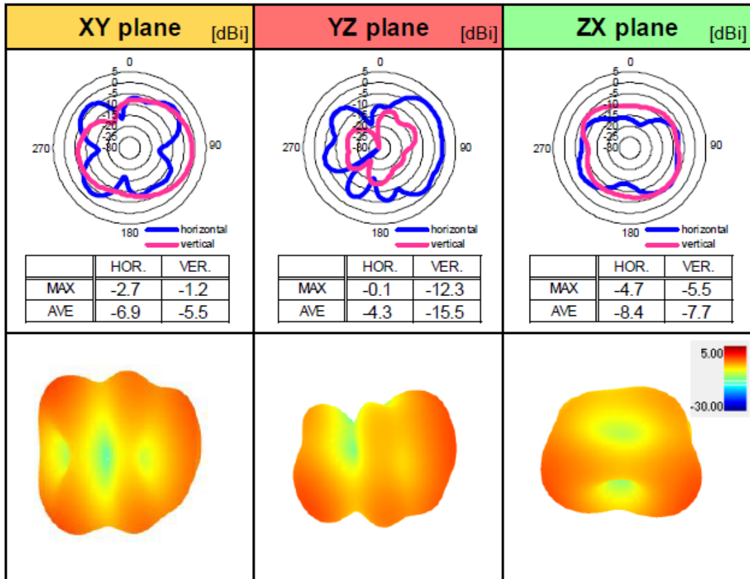
Figure 7 – 3D Directivity Measurements in 2 GHz Band
