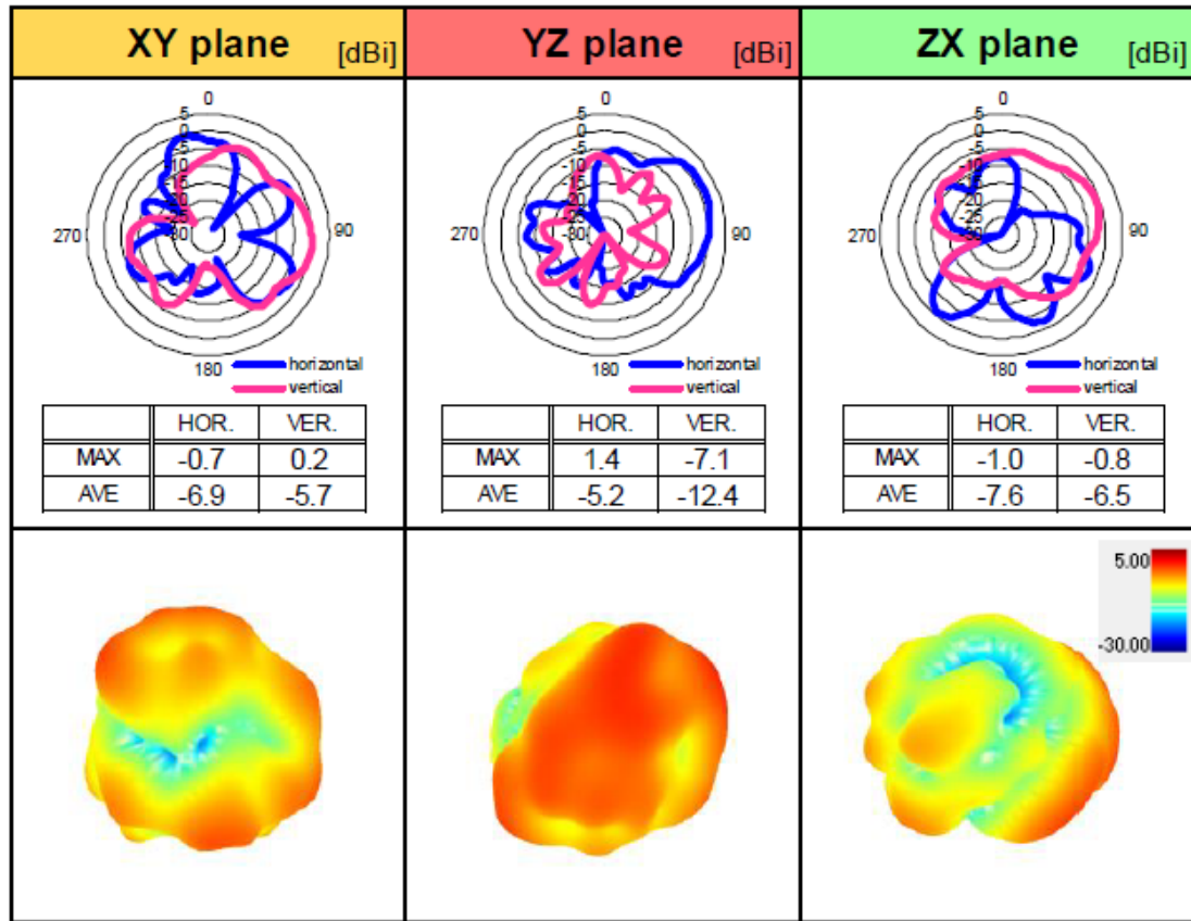
Figure 8 – 3D Directivity Measurements in 5 GHz Band
