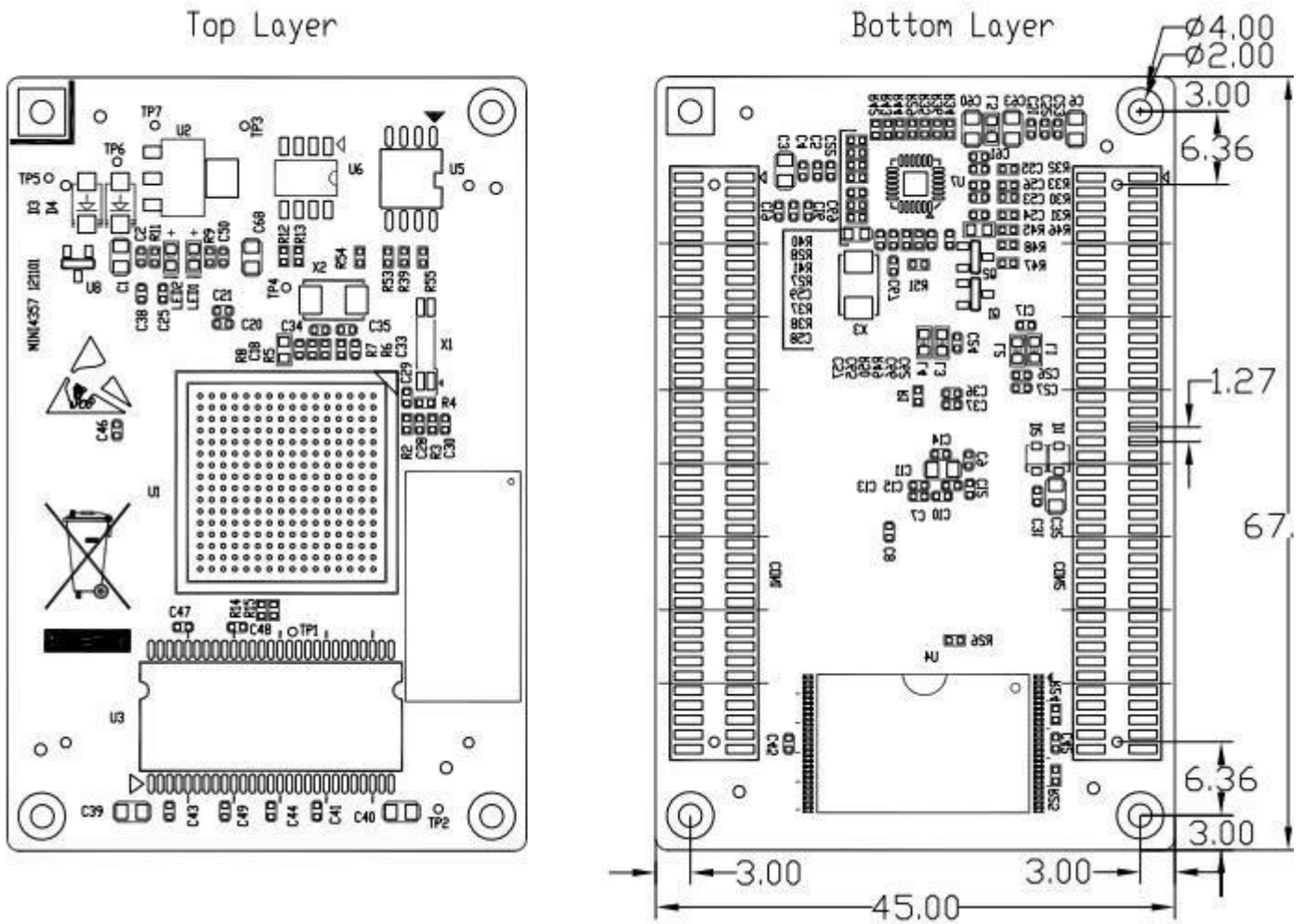
Hardware dimensions
