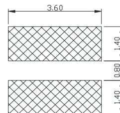
Recommand Pad Layout
