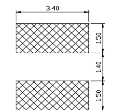
Recommend Pad Layout 1
