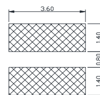
Recommend Pad Layout
