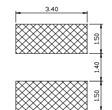
Recommend Pad Layout 1
