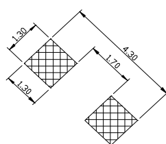
Recommend Pad Layout 2
