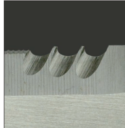
U-shaped blade
