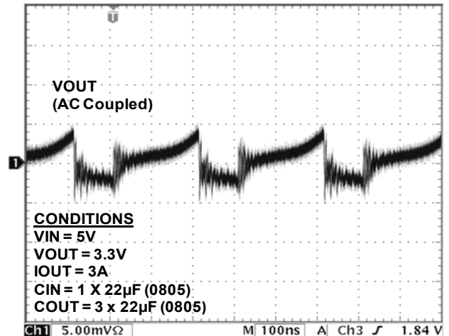
Output Ripple at 500MHz
