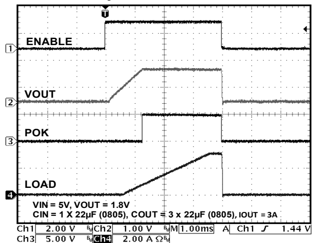
Startup Waveforms at 3A
