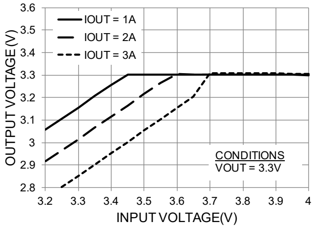
Dropout Voltage
