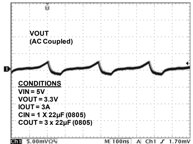
Output Ripple at 20MHz
