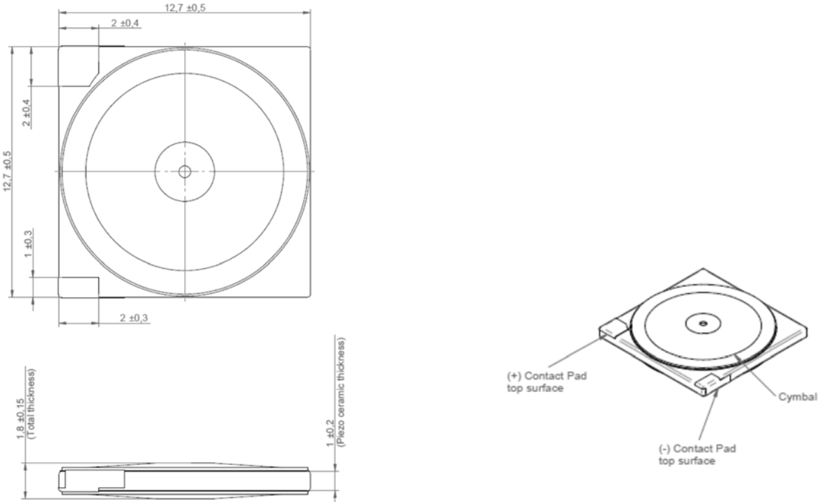
Fig. 1: Dimensional drawings
