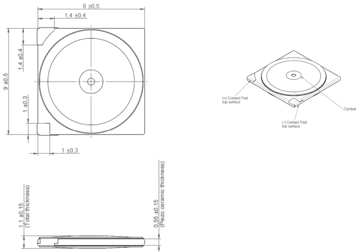
Fig. 1: Dimensional drawings
