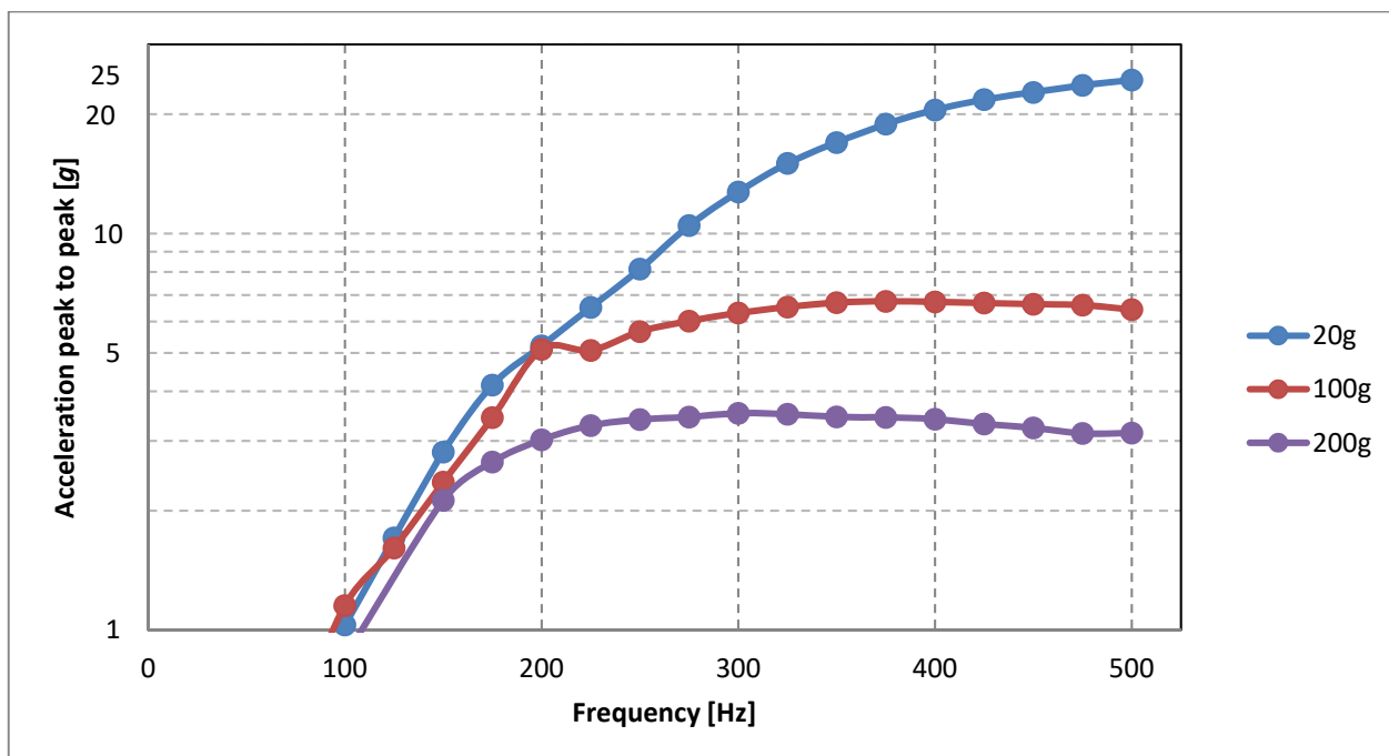
Fig. 7: Acceleration g as a function of frequency for different loads. Input voltage has a single pulse half wave sinus signal form of amplitude 0 ... 60 V and varying frequency from 50 ... 500 Hz.
