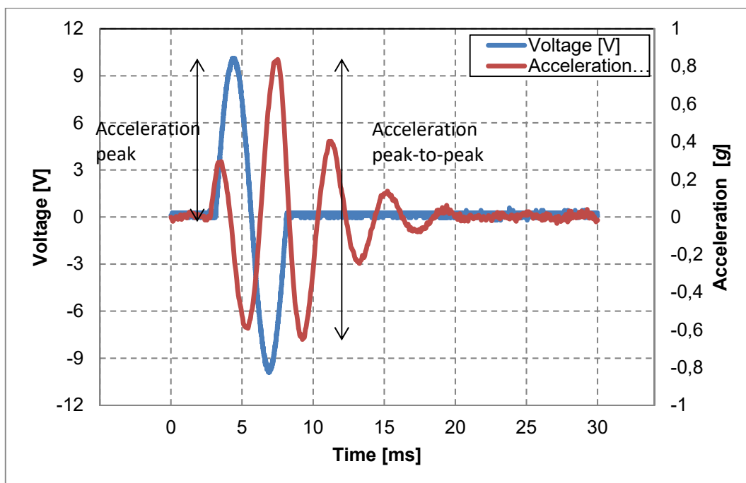
Fig. 6: Typical acceleration g as a function of input voltage with 100 g load. Input voltage with a sinus signal form of amplitude -10 ... 10 V and pulse length 5 ms which is equivalent to 200 Hz.
