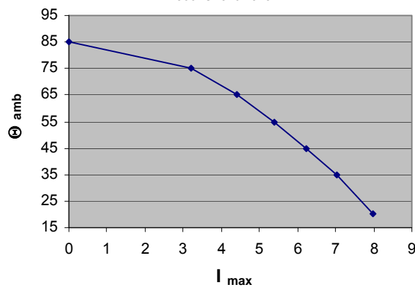
Max. allowable ambient Temp. at specific current (rms) B25667C7376A375
