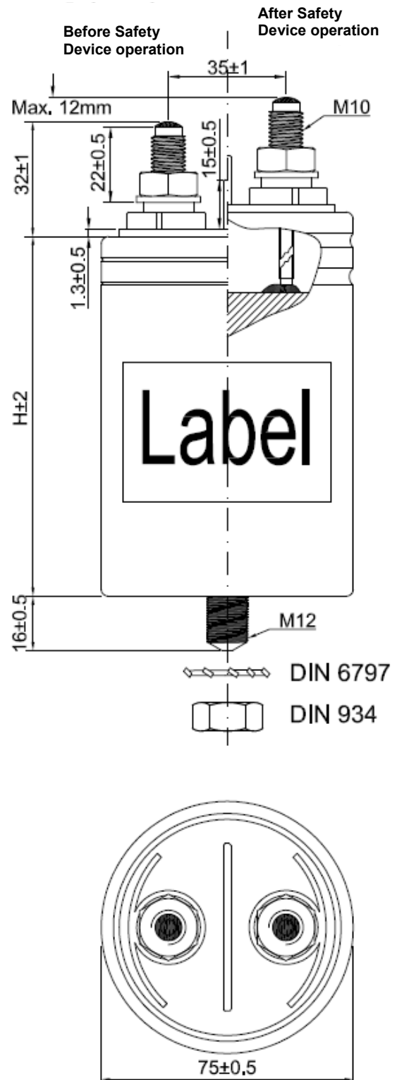
Figure 3: Series B32362
