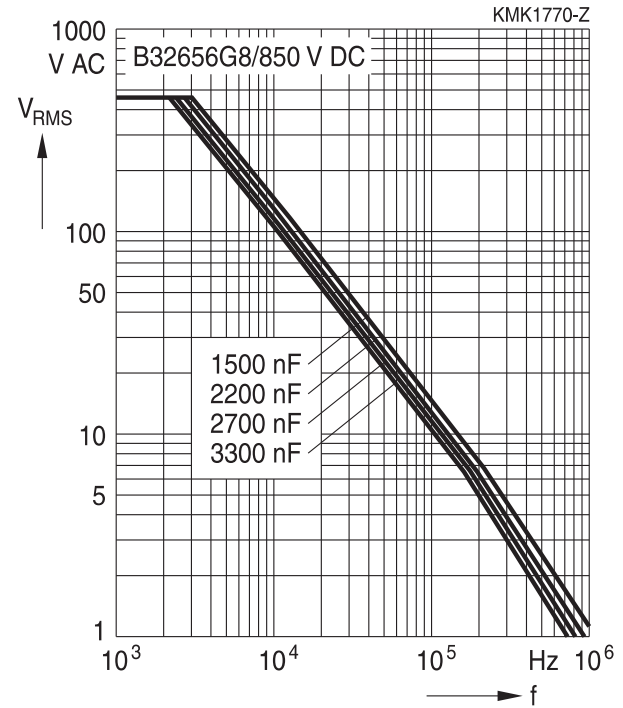
850 V DC/450 V AC, B32656G8
