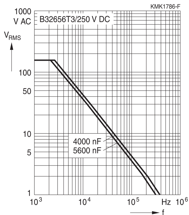
250 V DC/160 V AC, B32656T3
