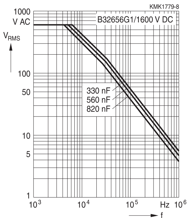
1600 V DC/600 V AC, B32656G1
