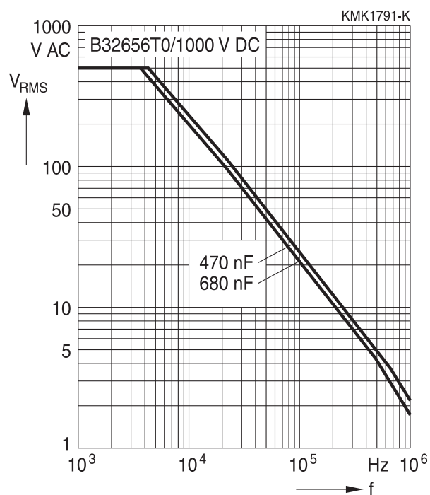
1000 V DC/500 V AC, B32656T0
