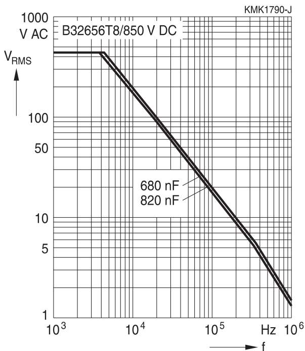
850 V DC/450 V AC, B32656T8
