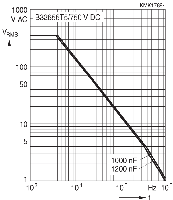
750 V DC/350 V AC, B32656T5
