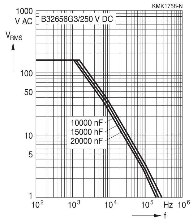
250 V DC/160 V AC, B32656G3
