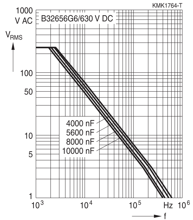
630 V DC/250 V AC, B32656G6
