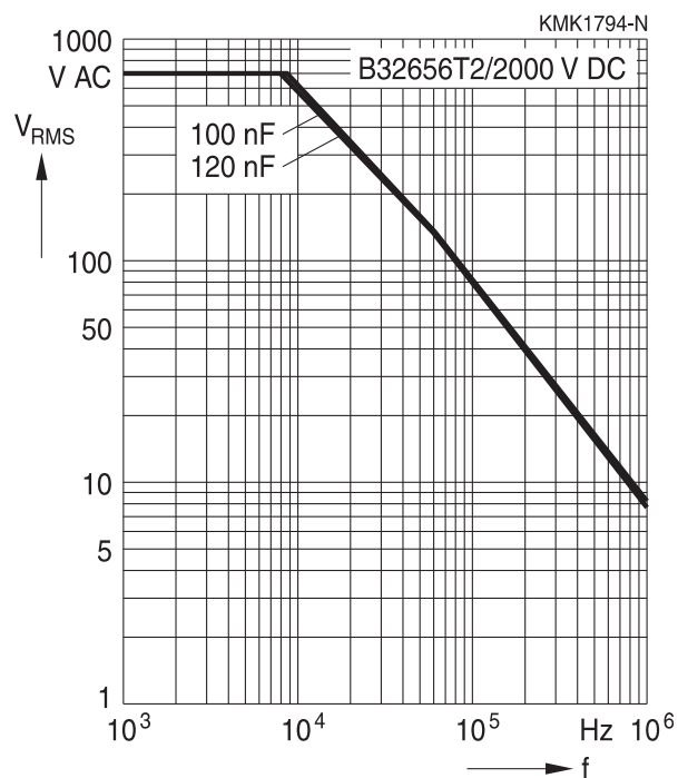
2000 V DC/700 V AC, B32656T2
