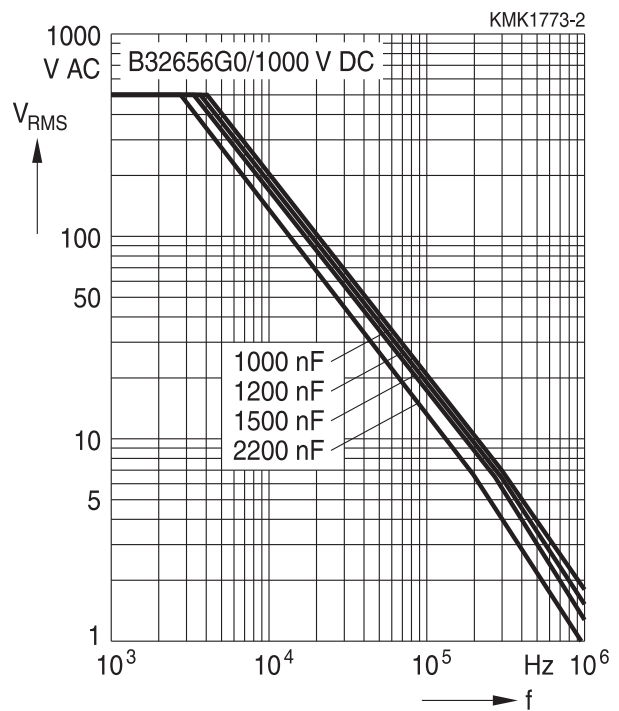
1000 V DC/500 V AC, B32656G0
