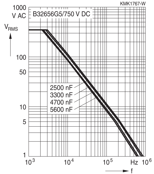
750 V DC/350 V AC, B32656G5
