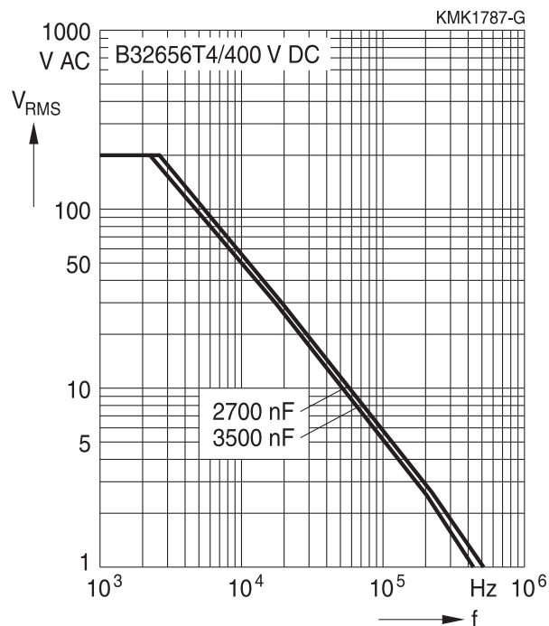
400 V DC/200 V AC, B32656T4
