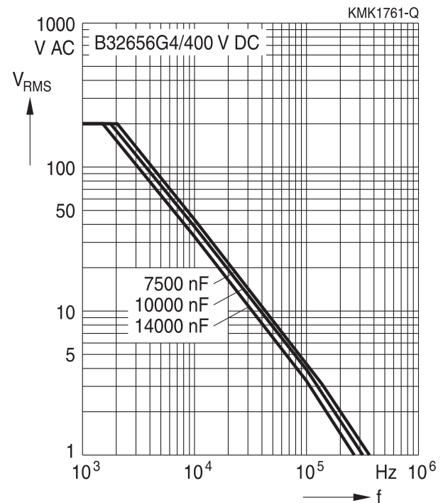
400 V DC/200 V AC, B32656G4
