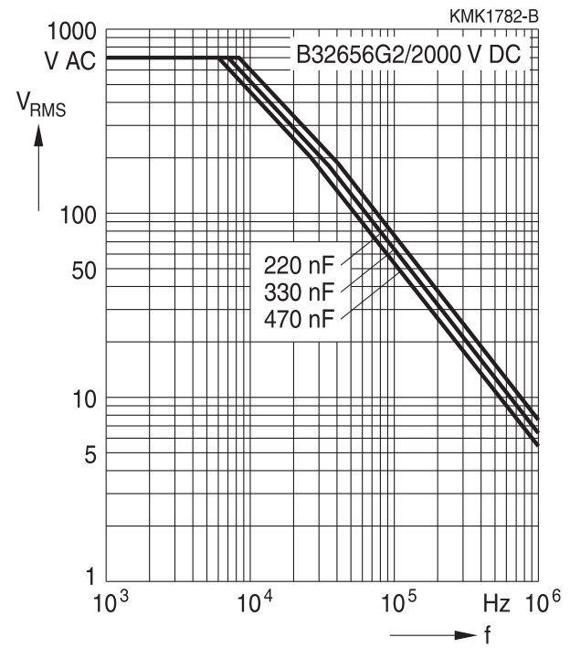
2000 V DC/700 V AC, B32656G2
