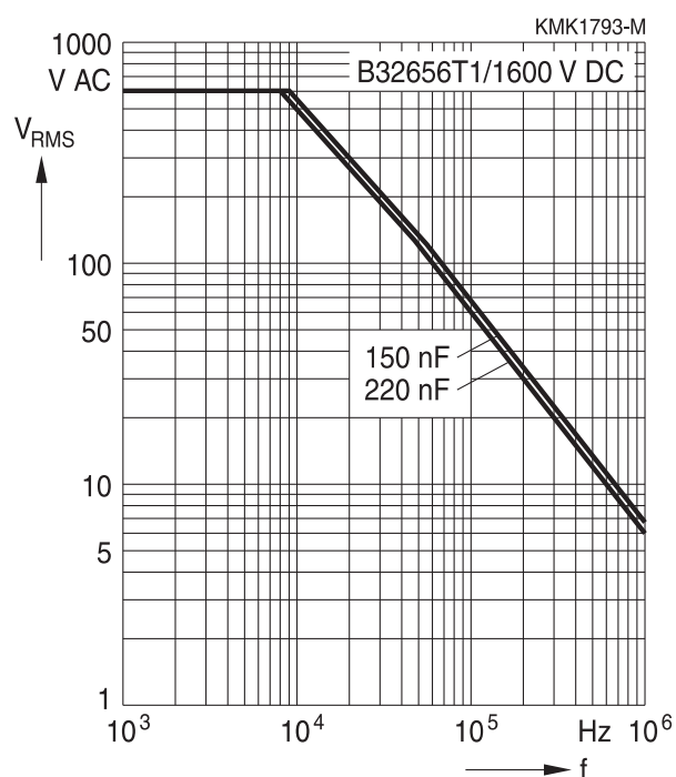
1600 V DC/600 V AC, B32656T1
