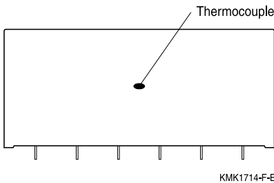
Figure 2 (12-pin)
