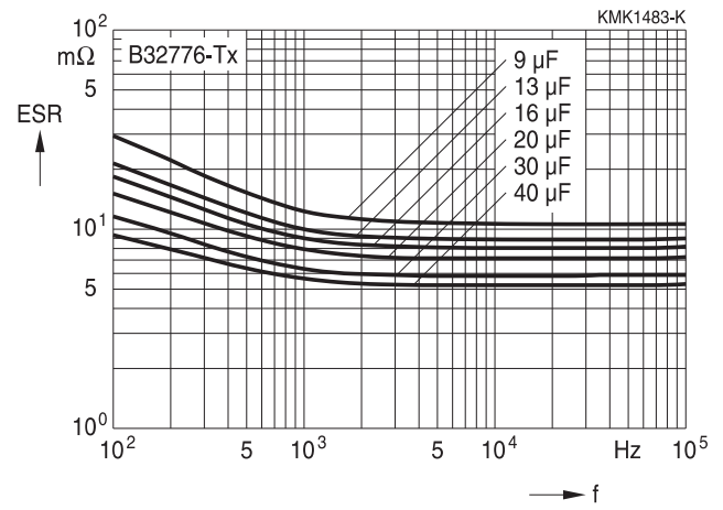
ESR versus frequency f (typical values)
