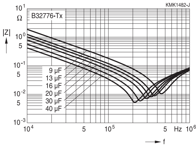
Impedance Z versus frequency f (typical values)
