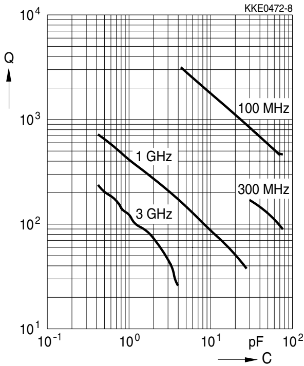
Q factor versus capacitance C
