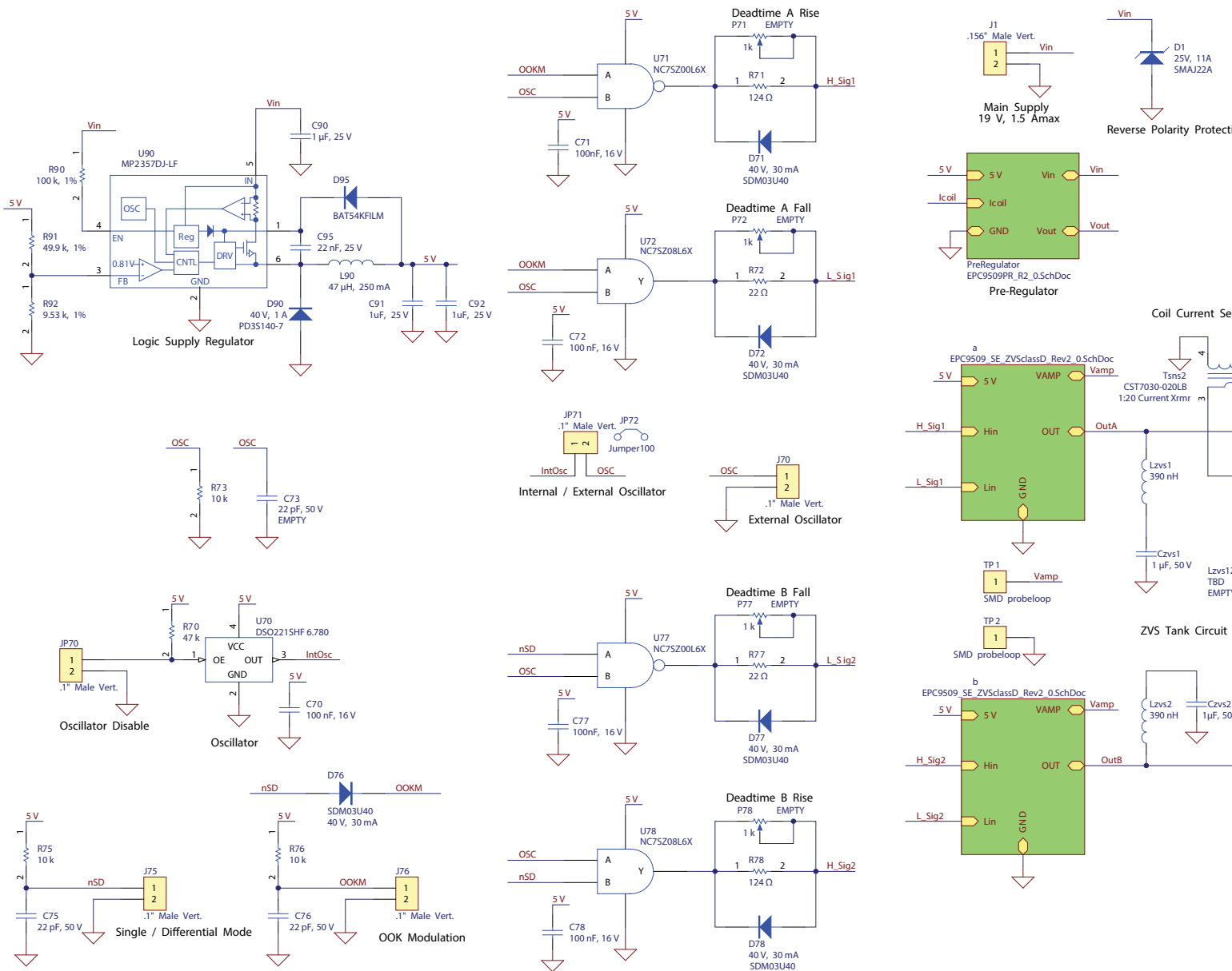
Figure 13: EPC9509 - Pre-regulator schematic.
