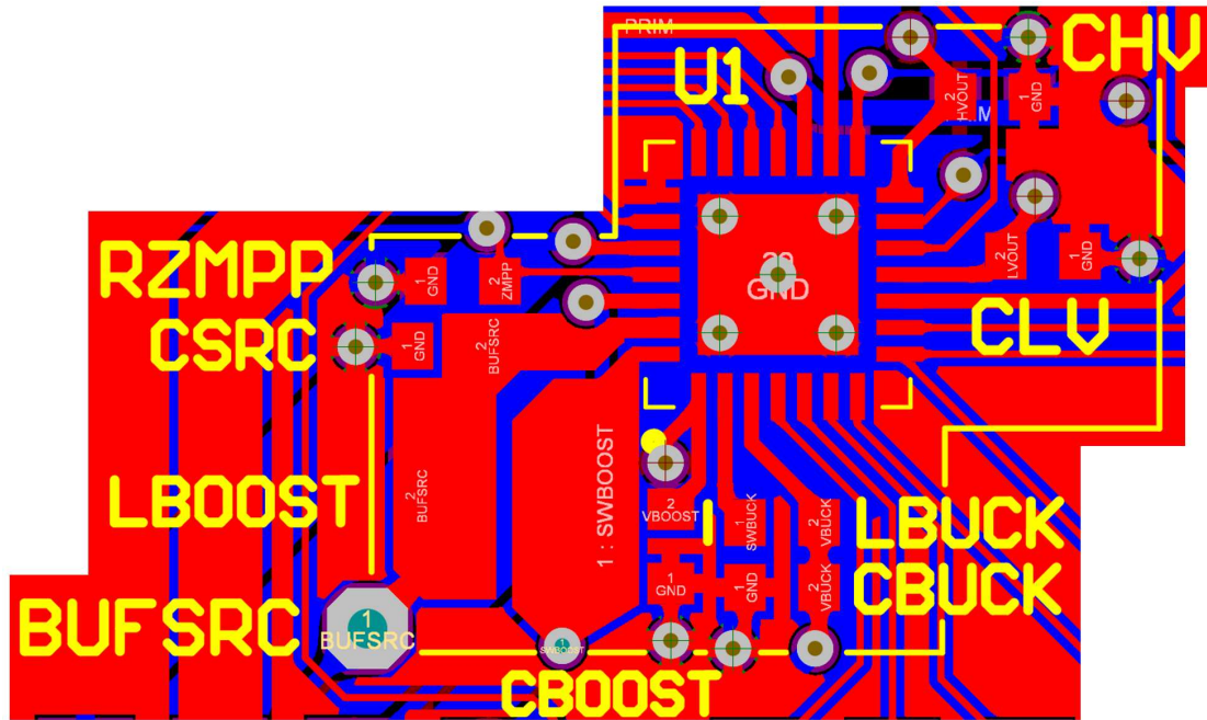
Figure 21: Layout example for the AEM20940 and its passive components
