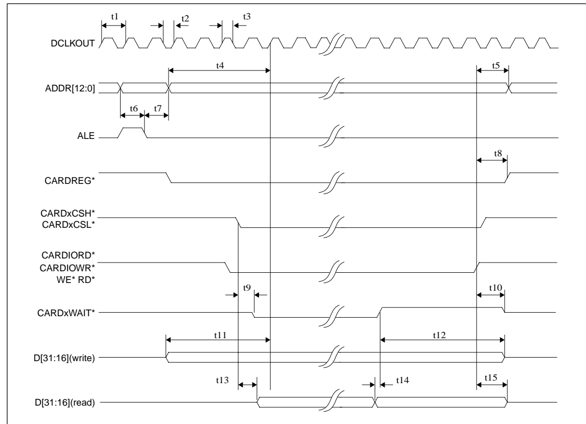
Figure 7-10 Toshiba Timing
