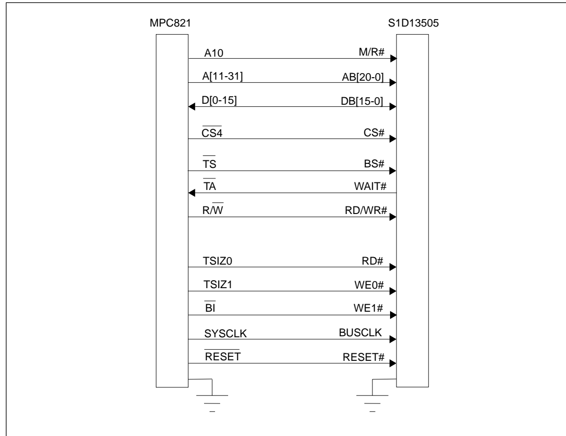
Figure 6-1 Schematic for MPC821/S1D13505 Interface
