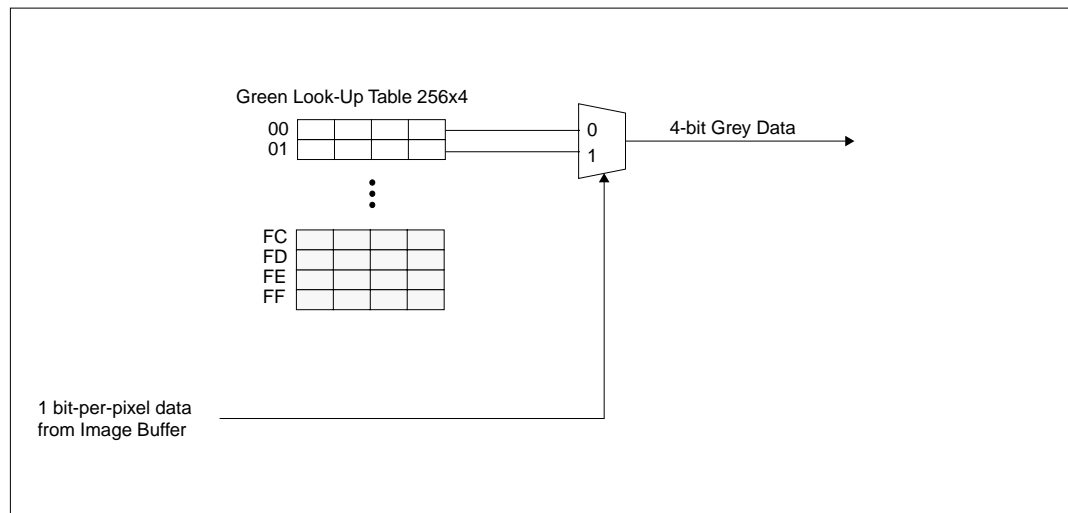
Figure 11-1 1 Bit-per-pixel Monochrome Mode Data Output Path
