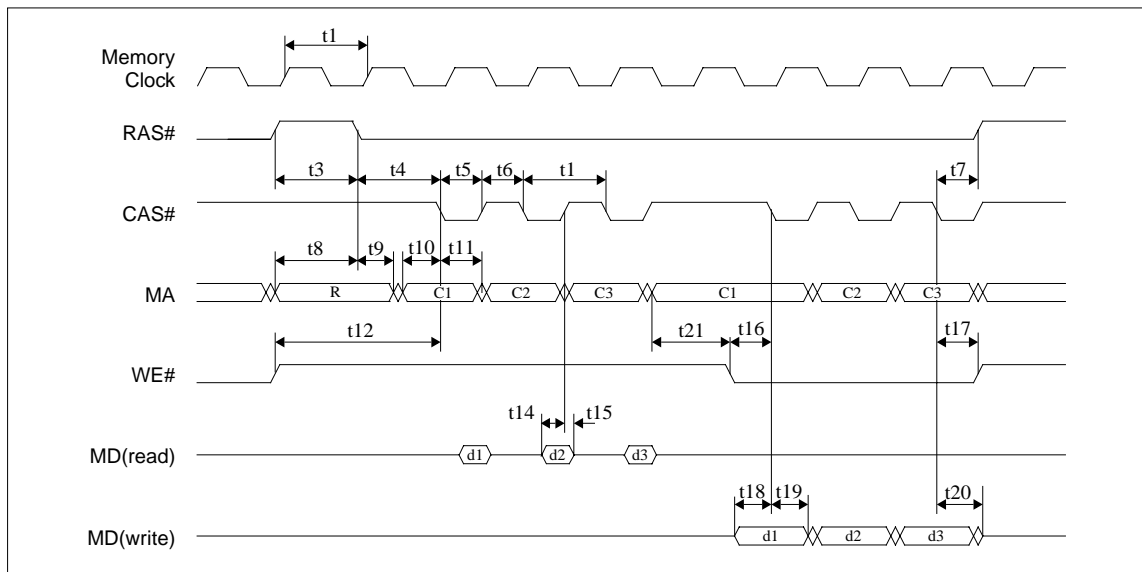
Figure 7-19 FPM-DRAM Read-Write Timing
