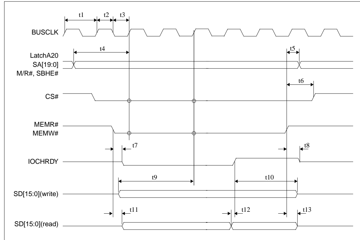
Figure 7-7 MIPS/ISA Timing
