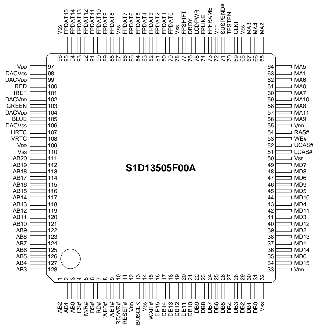
Figure 5-1 Pinout Diagram
