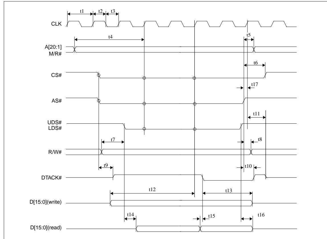
Figure 7-3 MC68000 Timing
