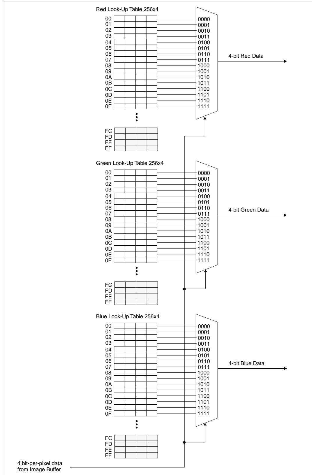
Figure 11-6 4 Bit-per-pixel Color Mode Data Output Path
