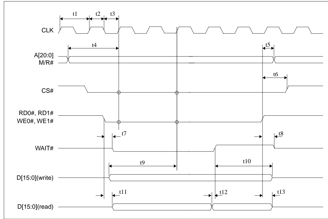
Figure 7-6 Generic Timing
