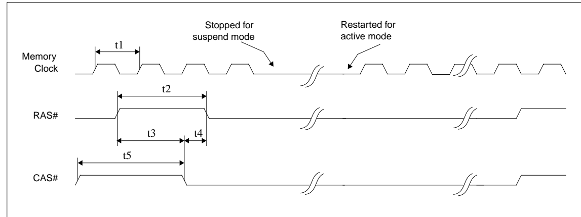
Figure 7-17 EDO-DRAM Self-Refresh Timing
