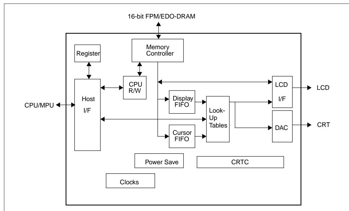
Figure 4-1 System Block Diagram Showing Datapaths
