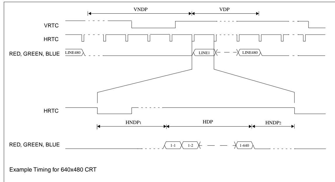
Figure 7-44 CRT Timing
