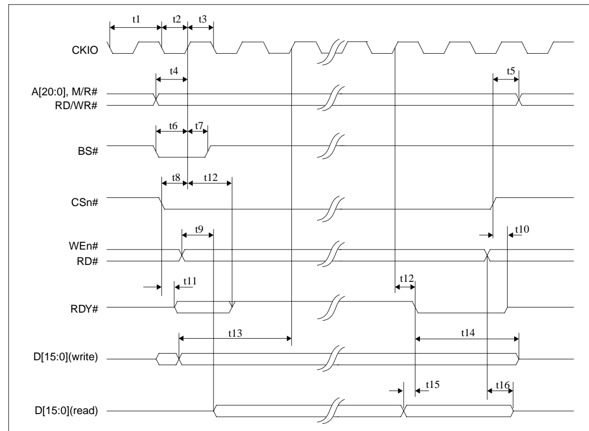
Figure 7-1 SH-4 Timing
