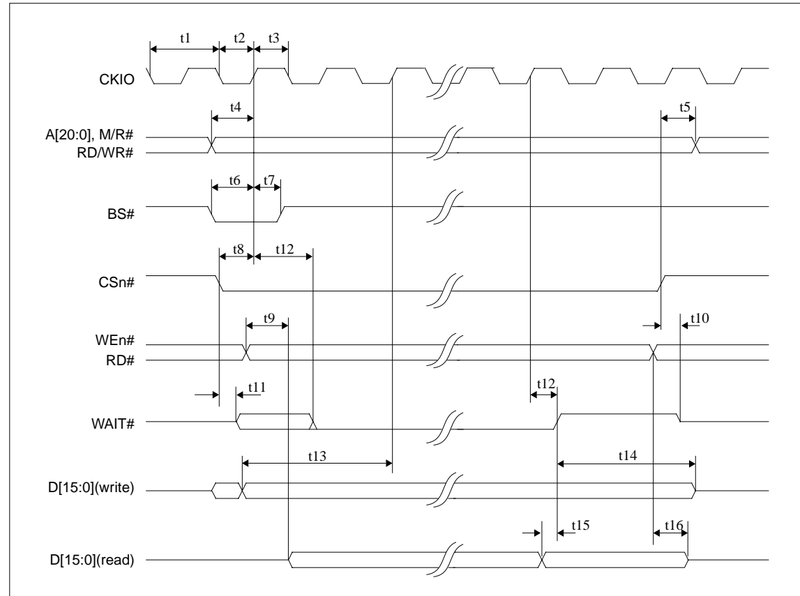
Figure 7-2 SH-3 Timing
