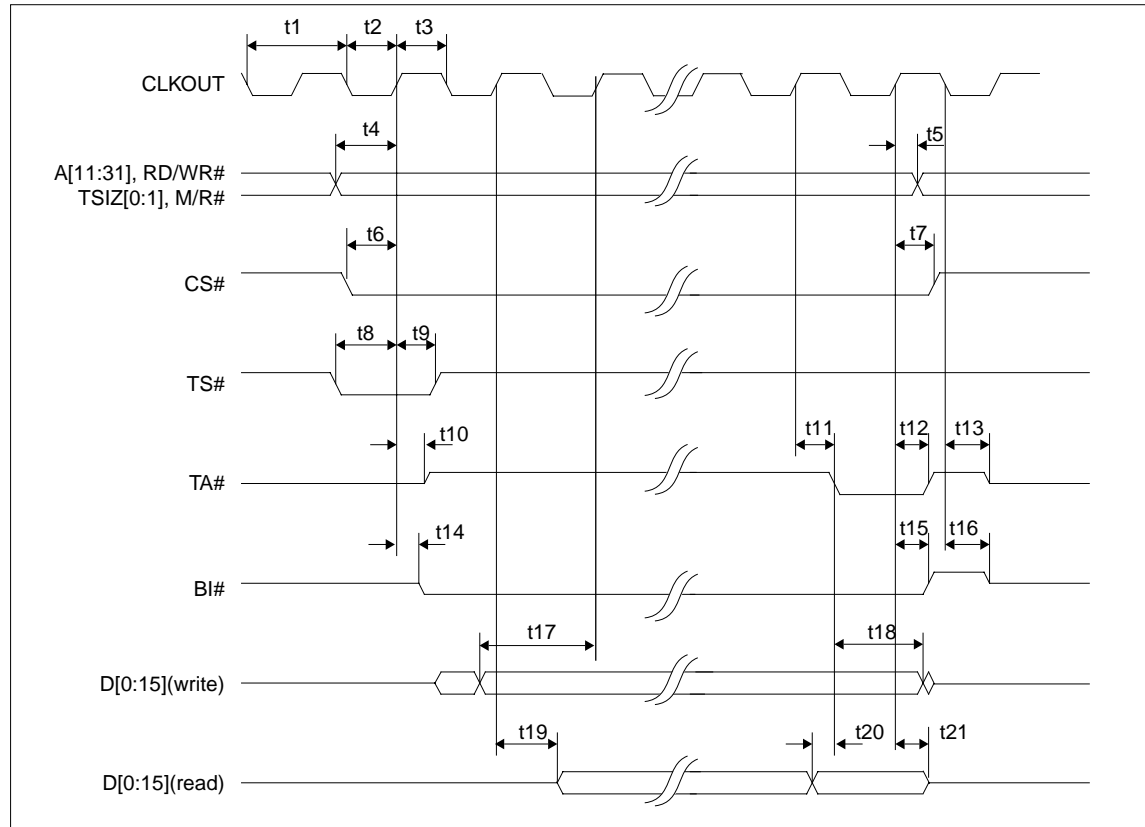
Figure 7-12 PowerPC Timing
