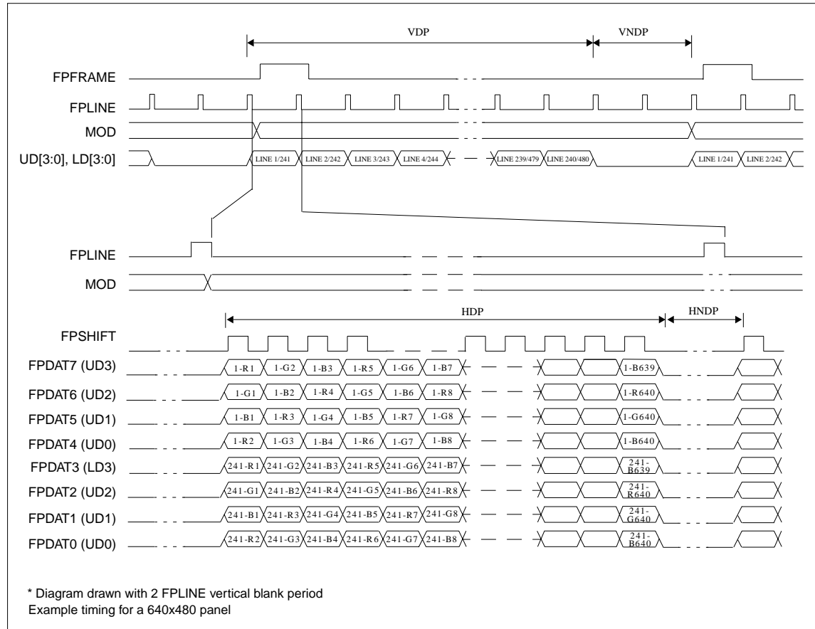
Figure 7-38 8-Bit Dual Color Passive LCD Panel Timing
