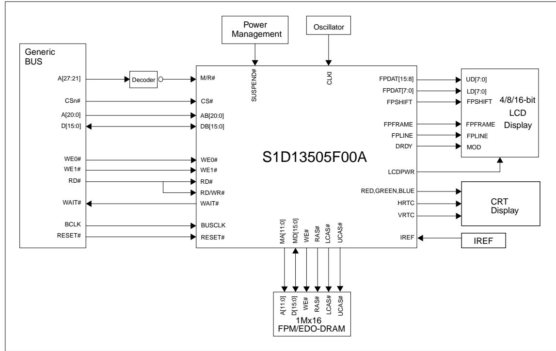
Figure 3-5 Typical System Diagram (Generic Bus, 1Mx16 FPM/EDO-DRAM)
