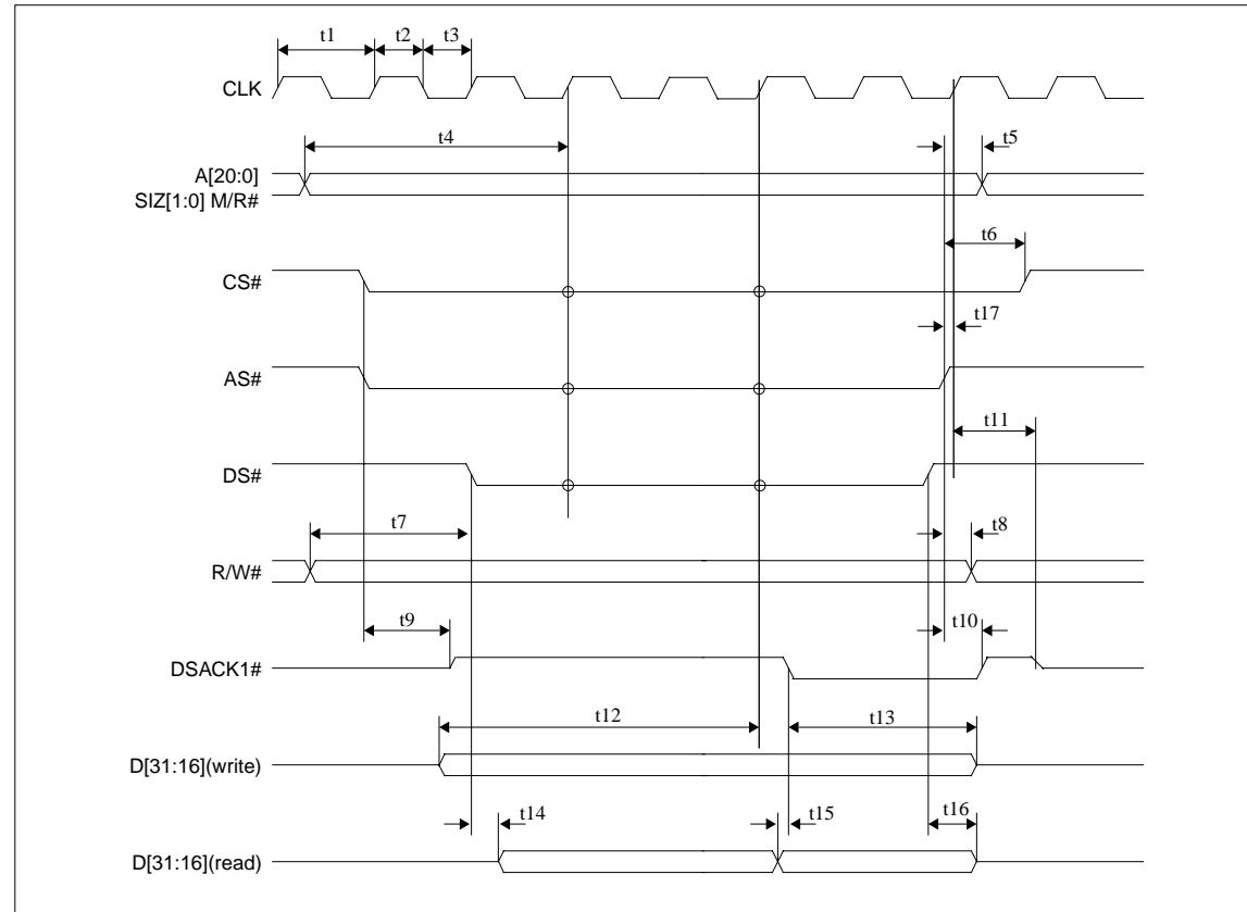
Figure 7-4 MC68030 Timing
