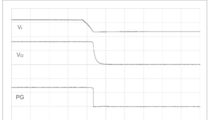
Shut-down by removing V_i . V_i = 12\text{ V} , I_o = \text{max } I_o , PG pulled up to V_o . Scale: 10 or 1 V/div, 1 ms/div.
