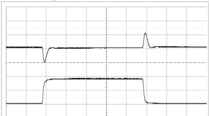
Output voltage response to load current step change (4.5–13.5–4.5 A) at V_I = 12\text{ V} , C_O = 3 \times 100\ \mu\text{F} + 270\ \mu\text{F}/10\text{m}\Omega . Default compensation settings. Scale: 50 mV/div, 5 A/div, 100 \mu\text{s} /div.
