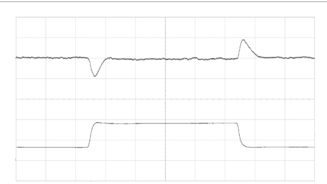
Output voltage response to load current step change (3–9–3 A) at V_i = 12\text{ V} , C_o = 3 \times 100\ \mu\text{F} + 270\ \mu\text{F}/10\text{m}\Omega . Default compensation settings. Scale: 50 mV/div, 5 A/div, 50 \mu\text{s} /div.
