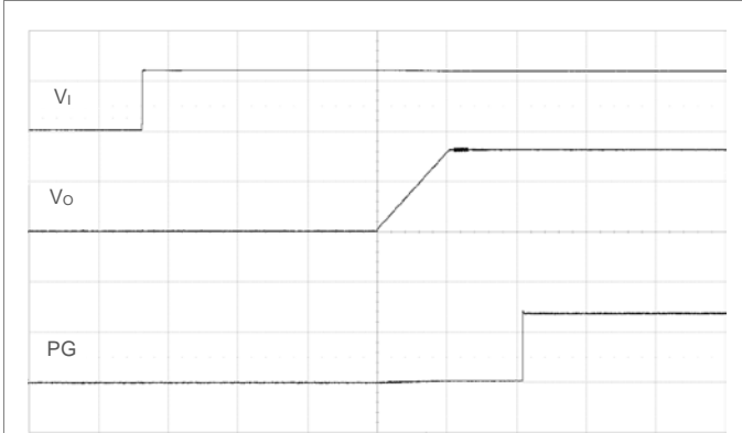
Start-up enabled by applying V_i . T_{ON\_DELAY} = T_{ON\_RISE} = 10\text{ ms} (default). V_i = 12\text{ V} , I_o = \text{max } I_o , PG pulled up to V_o . Scale: 10 or 1 V/div, 10 ms/div. V_{out}=1.8\text{V}
