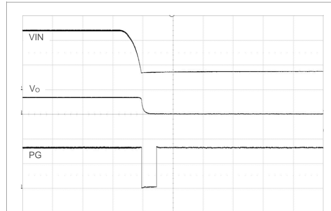
Shut-down by removing V_{in} . V_i = 12\text{ V} , I_o = \text{max } I_o , PG pulled up to external 3.3V. Scale: 10 or 5 V/div, 1 ms/div. V_{out}=3.3\text{V}
