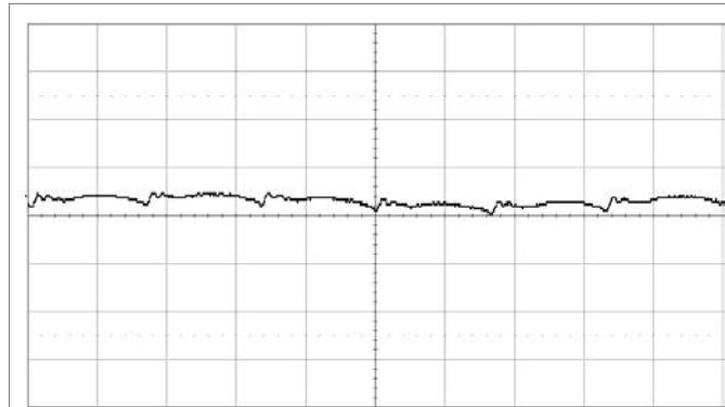
Fundamental output voltage ripple at V_I = 12\text{ V} , C_O = 3 \times 100\ \mu\text{F} , I_O = 15\text{ A} . Scale: 5 mV/div, 1 \mu\text{s} /div, 20 MHz bandwidth. See section Output Ripple and Noise.
