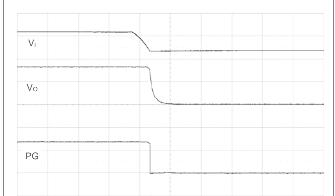
Shut-down by removing V_i . V_i = 12\text{ V} , I_o = \text{max } I_o , PG pulled up to V_o . Scale: 10 or 2 V/div, 1 ms/div.
