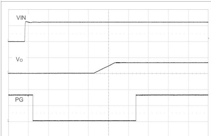
Start-up enabled by applying V_{in} . T_{ON\_DELAY} = T_{ON\_RISE} = 10\text{ ms} (default). V_i = 12\text{ V} , I_o = \text{max } I_o , PG pulled up to external 3.3V. Scale: 10 or 5 V/div, 10 ms/div. V_{out}=3.3\text{V}
