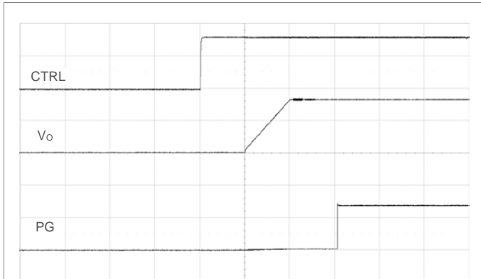
Start-up enabled by CTRL signal. \text{TON\_DELAY} = \text{TON\_RISE} = 10\text{ ms} (default). V_i = 12\text{ V} , I_o = \text{max } I_o , PG pulled up to V_o . Scale: 2 or 1 V/div, 10 ms/div.
