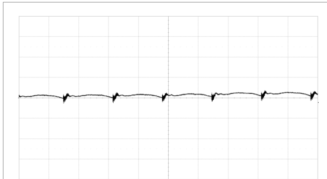
Fundamental output voltage ripple at V_i = 12\text{ V} , C_o = 3 \times 100\ \mu\text{F} , I_o = 12\text{ A} . Scale: 5 mV/div, 1 \mu\text{s} /div, 20 MHz bandwidth. See section Output Ripple and Noise.
