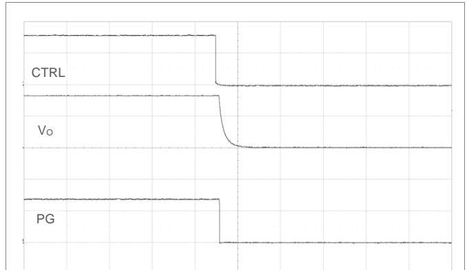
Shut-down by CTRL signal. V_i = 12\text{ V} , I_o = \text{max } I_o , PG pulled up to V_o . Scale: 2 or 1 V/div, 1 ms/div.
