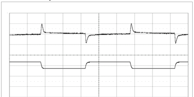
Output voltage response to load current step change (1.5–4.5–1.5 A) at V_i = 12\text{ V} , C_o = 3 \times 100\ \mu\text{F} + 270\ \mu\text{F}/10\text{m}\Omega . Default compensation settings. Scale: 20 mV/div, 5 A/div, 100 \mu\text{s} /div.
