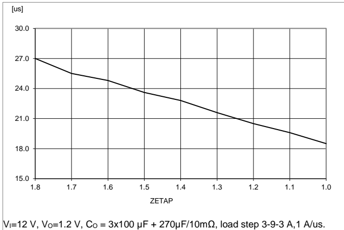
Recovery time to within 1% of V_O vs. ZETAP setting.
