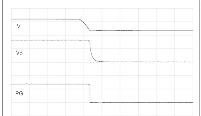
Shut-down by removing V_i . V_i = 12\text{ V} , I_o = \text{max } I_o , PG pulled up to V_o . Scale: 10 or 1 V/div, 1 ms/div. V_{out}=1.8\text{V}
