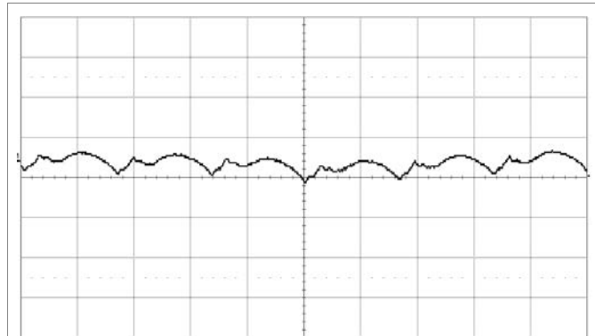
Fundamental output voltage ripple at V_I = 12\text{ V} , C_O = 3 \times 100\ \mu\text{F} , I_O = 18\text{ A} . Scale: 5 mV/div, 1 μs/div, 20 MHz bandwidth. See section Output Ripple and Noise.
