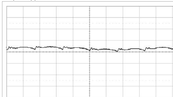
Fundamental output voltage ripple at V_I = 12\text{ V} , C_O = 3 \times 100\ \mu\text{F} , I_O = 18\text{ A} . Scale: 5 mV/div, 1 \mu\text{s} /div, 20 MHz bandwidth. See section Output Ripple and Noise.
