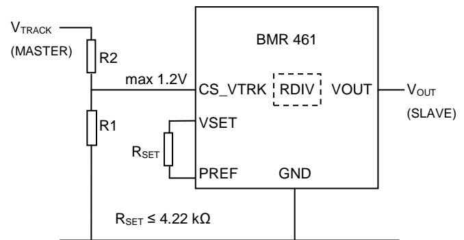
Tracking Mode Configuration
