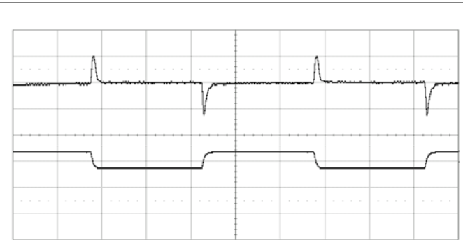
Output voltage response to load current step change (1.5–4.5–1.5 A) at V_i = 12\text{ V} , C_o = 3 \times 100\ \mu\text{F} + 270\ \mu\text{F}/10\text{m}\Omega . Default compensation settings. Scale: 20 mV/div, 5 A/div, 100 \mu\text{s} /div.
