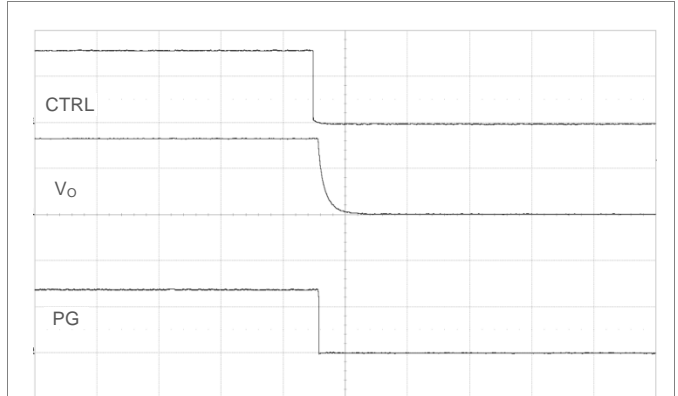
Shut-down by CTRL signal. V_i = 12\text{ V} , I_o = \text{max } I_o , PG pulled up to V_o . Scale: 2 V/div, 1 ms/div.
