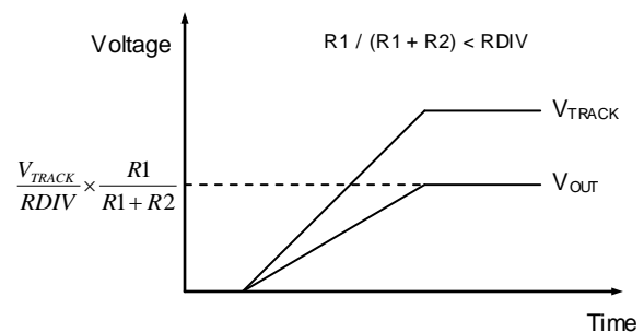
Ratiometric Voltage Tracking
