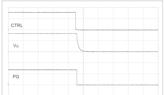
Shut-down by CTRL signal. V_i = 12\text{ V} , I_o = \text{max } I_o , PG pulled up to V_o . Scale: 2 or 1 V/div, 1 ms/div. V_{out}=1.8\text{V}
