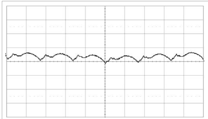
Fundamental output voltage ripple at V_i = 12\text{ V} , C_o = 3 \times 100\ \mu\text{F} , I_o = 15\text{ A} . Scale: 5 mV/div, 1 μs/div, 20 MHz bandwidth. See section Output Ripple and Noise.
