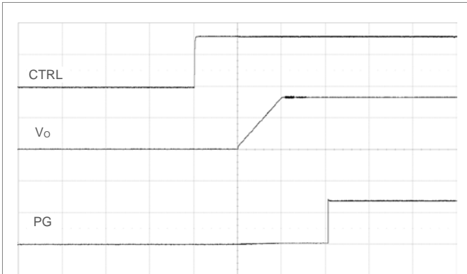
Start-up enabled by CTRL signal. T_{ON\_DELAY} = T_{ON\_RISE} = 10\text{ ms} (default). V_i = 12\text{ V} , I_o = \text{max } I_o , PG pulled up to V_o . Scale: 2 or 1 V/div, 10 ms/div. V_{out}=1.8\text{V}
