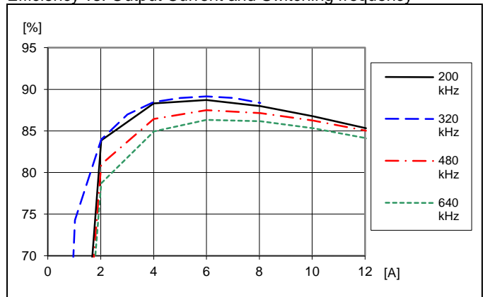
Efficiency vs. load current and switching frequency at T_{P1} = +25^\circ C . V_i = 12 V , V_o = 3.3 V , C_o = 470 \mu F / 10 m\Omega Default configuration except changed frequency
