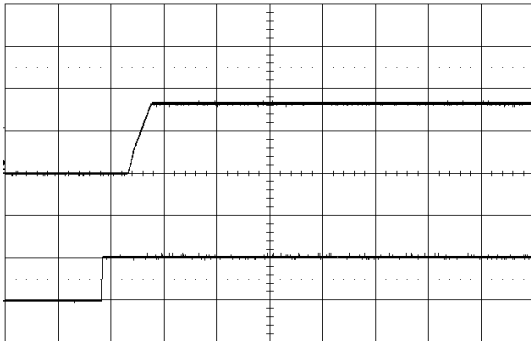
Start-up by enabling CTRL signal at: T_{P1} = +25^\circ\text{C} , V_I = 12\text{ V} , V_O = 3.3\text{ V} C_O = 470\ \mu\text{F}/10\ \text{m}\Omega , I_O = 12\text{ A} Top trace: output voltage (2 V/div.). Bottom trace: CTRL signal (2 V/div.). Time scale: (20 ms/div.).
