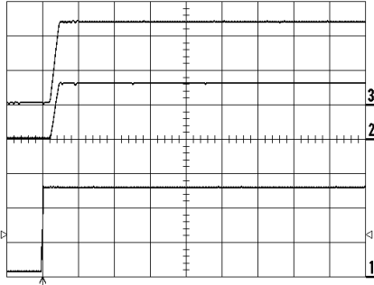
Start-up enabled by connecting V_i at: T_{ref} = +25^{\circ}\text{C} , V_i = 53\text{ V} , I_{O1} = 1.5\text{ A} , I_{O2} = 1.4\text{ A} resistive load. Top trace: output voltage 2 (2.0 V/div.). Mid trace: output voltage 1 (2.0 V/div.). Bottom trace: input voltage (20 V/div.). Time scale: (10 ms/div.).
