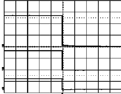
Shut-down enabled by disconnecting V_i at: T_{ref} = +25^{\circ}\text{C} , V_i = 53\text{ V} , I_{O1} = 1.5\text{ A} , I_{O2} = 1.4\text{ A} resistive load. Bottom trace: output voltage 2 (5.0 V/div.). Mid trace: output voltage 1 (2.0 V/div.). Top trace: input voltage (20 V/div.). Time scale: (100 ms/div.).
