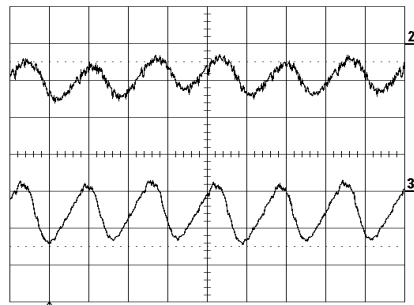
Output voltage ripple at: T_{ref} = +25^{\circ}\text{C} , V_i = 53\text{ V} , I_{O1} = 1.5\text{ A} , I_{O2} = 1.4\text{ A} resistive load. Top trace: output voltage 1 (2 mV/div.). Bottom trace: output voltage 2 (5 mV/div.). Time scale: (2 \mu\text{s} /div.).
