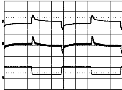
Output voltage response to load current step-change, output 1 (0.375-1.125-0.375 A) at: T_{ref} = +25^{\circ}\text{C} , V_i = 53\text{ V} , I_{O2} = 1.4\text{ A} . Top trace: output voltage 2 (200 mV/div.). Mid trace: output voltage 1 (200 mV/div.). Bottom trace: load current (1.0 A/div.). Time scale: (0.2 ms/div.).
