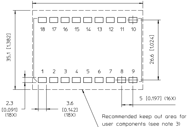
FOOTPRINT (top view, application board) 48.8 [1.921]
