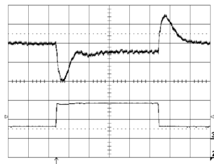
Output voltage response to load current step-change (0.3-0.9-0.3 A) at: T_{ref} = +25^\circ\text{C} , V_i = 53\text{ V} .
