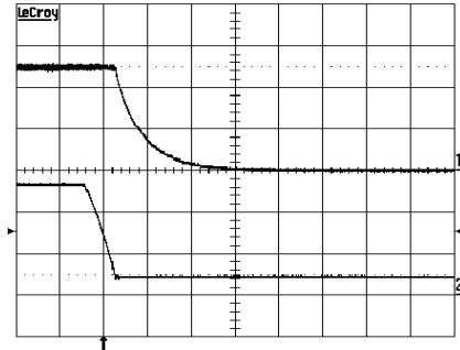
Shut-down enabled by disconnecting V_i at: T_{ref} = +25^\circ\text{C} , V_i = 53\text{ V} , I_o = 1.2\text{ A} resistive load.
