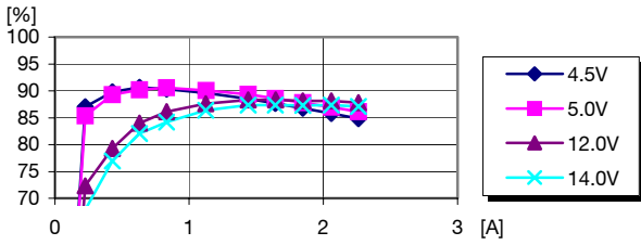
Efficiency vs. load current and input voltage at T_{ref} = +25^{\circ}C
