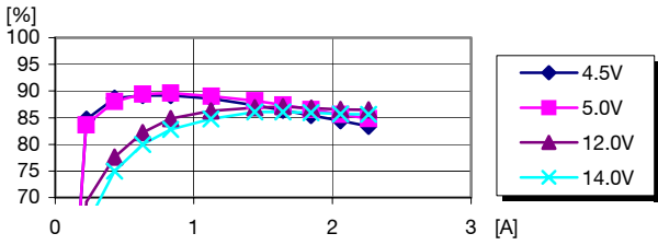
Efficiency vs. load current and input voltage at T_{ref} = +25^{\circ}C
