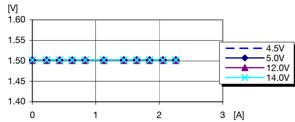
Output voltage vs. load current at T_{ref} = +25^{\circ}C
