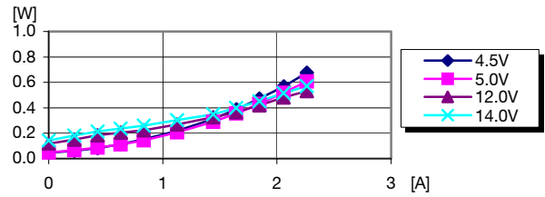
Dissipated power vs. load current and input voltage at T_{ref} = +25^{\circ}C
