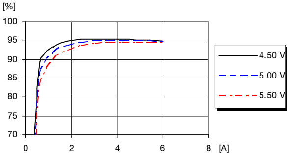
Efficiency vs. load current and input voltage at T_{ref} = +25^{\circ}C
