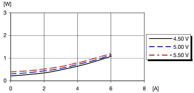
Dissipated power vs. load current and input voltage at T_{ref} = +25^{\circ}C
