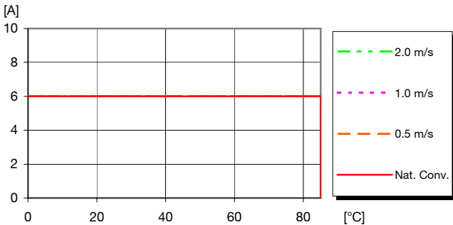
Available load current vs. ambient air temperature and airflow at V_I = 5.0 V, V_{OUT} = 3.3 V . See Thermal Consideration section.
