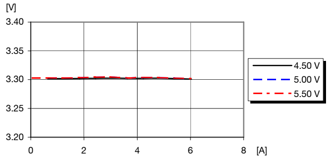
Output voltage vs. load current at T_{ref} = +25^{\circ}C
