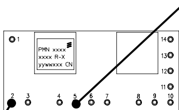
Pin 5 for measurement of minimum solder joint temperature, T_{PIN}
