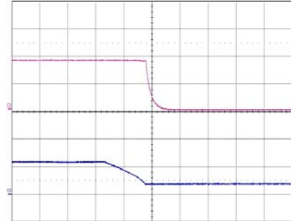
Shut-down enabled by disconnecting V_I at: T_{ref} = +25^\circ\text{C} , V_I = 12\text{ V} , Top trace: output voltage (1 V/div). Bottom trace: input voltage (10 V/div).
