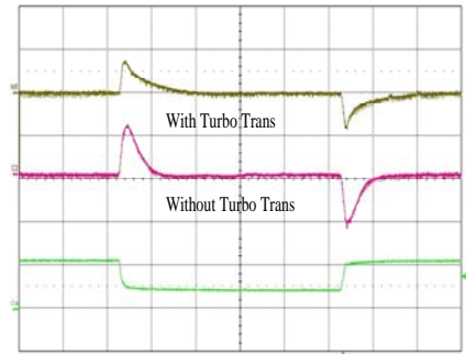
Output voltage response to load current step-change (7.5-22.5-7.5 A) at: T_{ref} = +25^\circ\text{C} , V_I = 12\text{ V} . Top trace: output voltage (100 mV/div). Middle trace: output voltage (100 mV/div). Bottom trace: load current (20 A/div).
