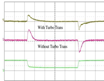
Output voltage response to load current step-change (7.5-22.5-7.5 A) at: T_{ref} = +25^\circ\text{C} , V_I = 12\text{ V} . Top trace: output voltage (100 mV/div). Middle Trace: output voltage (100mV/div). Bottom trace: load current (20 A/div).
