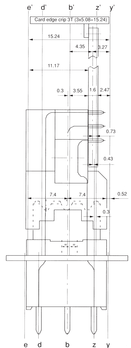
Exact position of connectors size F
