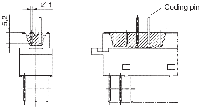
Female connector
