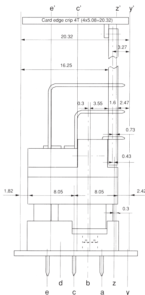
Exact position of connectors size E
