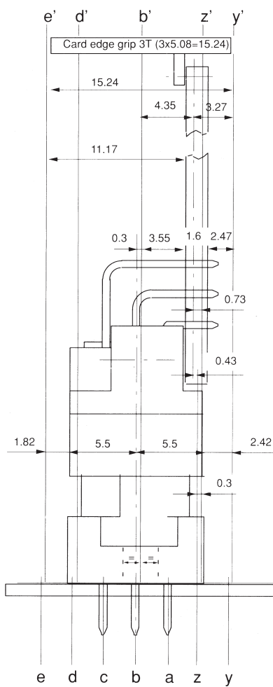
Exact position of connectors size C
