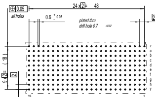
Board hole pattern (Component mounting side)
