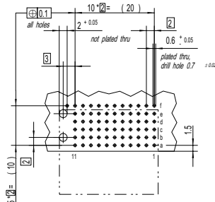
Board hole pattern (Component mounting side)
