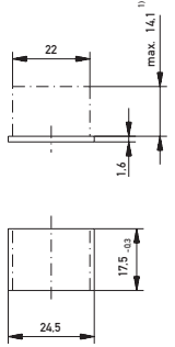
Querplatine / Crosswise circuit board
