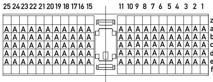
CONTACT LAYOUT
