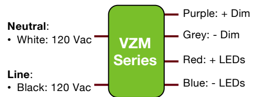
Wiring Diagram
