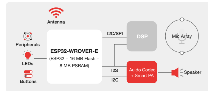
Hardware Architecture
