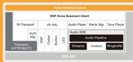
SDK Architecture
