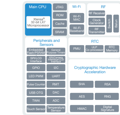
ESP32-S2 Block Diagram
