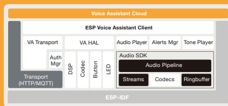
SDK Architecture
