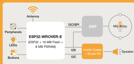
Hardware Architecture
