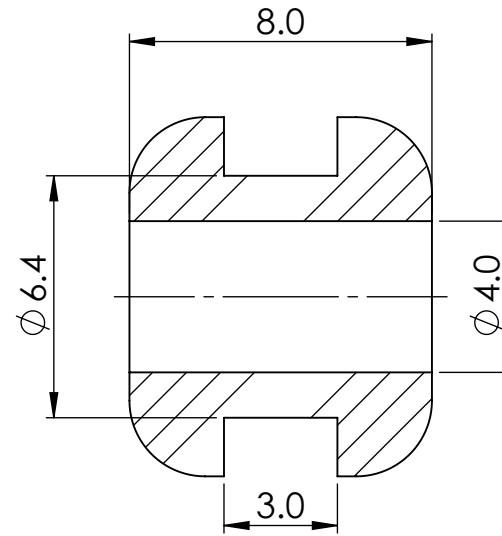
SECTION Y-Y
