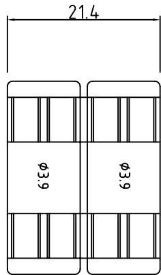
EFA04 71 P03 \phi 3.9 COUPLER CLIP
