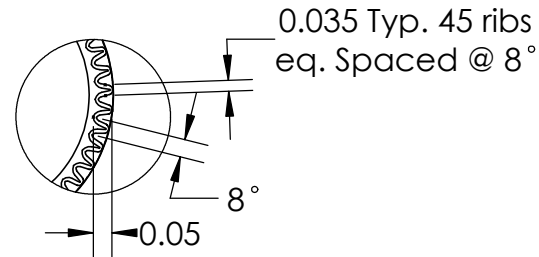
DETAIL B SCALE 1.5 : 1
