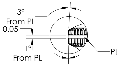
DETAIL C SCALE 1.5 : 1
