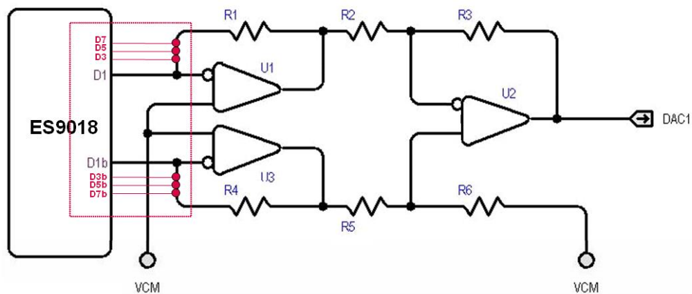
Sabre 32 Reference DAC in stereo “quad-differential” current mode (DNR: 133dB, THD: -120dB)
