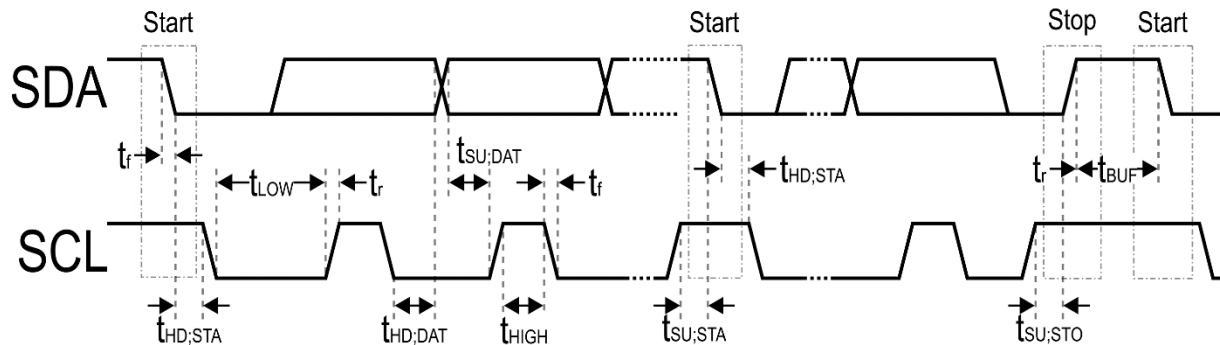
Figure 17 - I 2 C Slave Control Interface Timing
